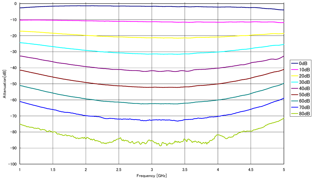
MAT800 Model A Attenuation(S21)
