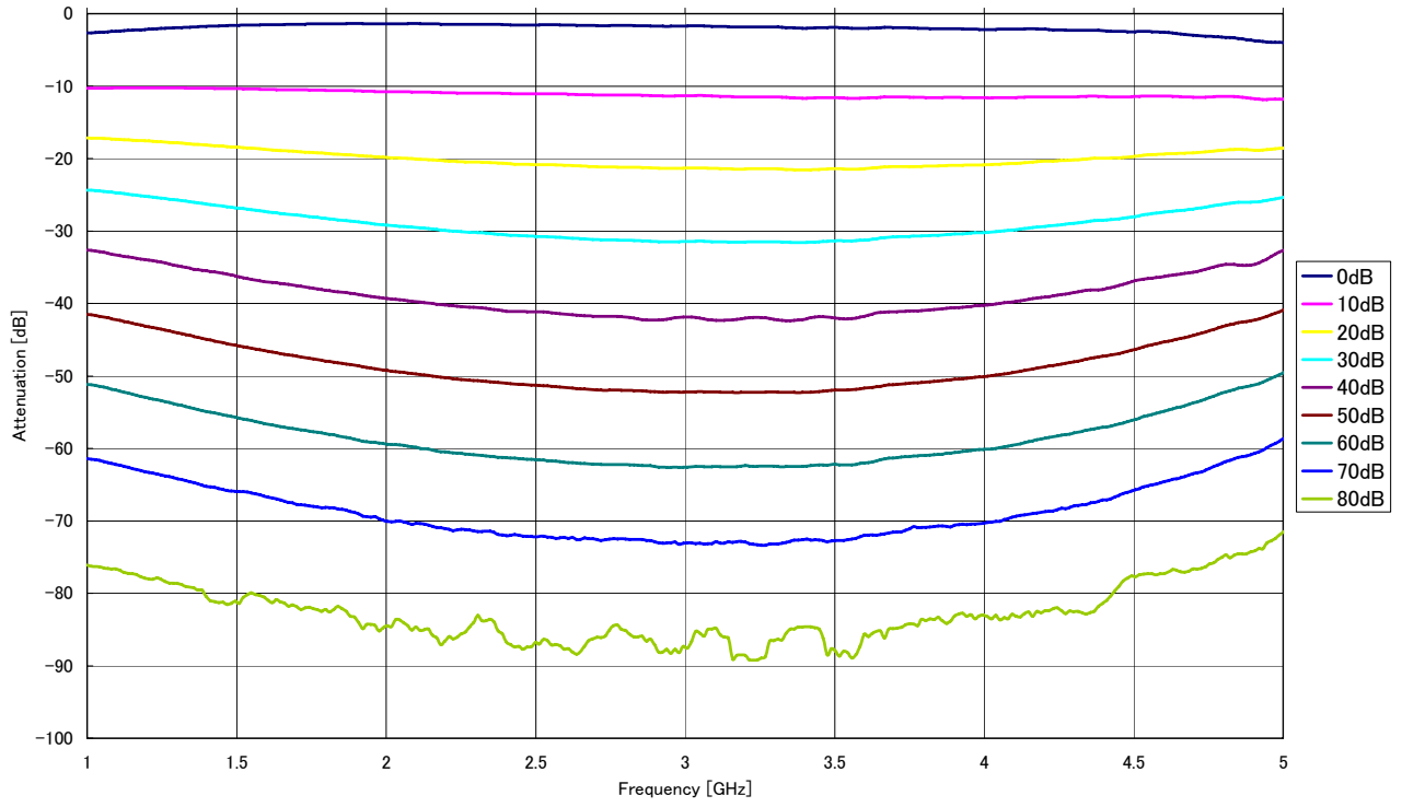
MAT800 Model A Attenuation(S12)
