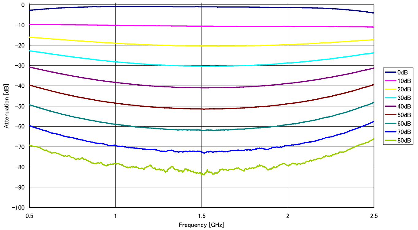
MAT800 Model E Attenuation(S21)
